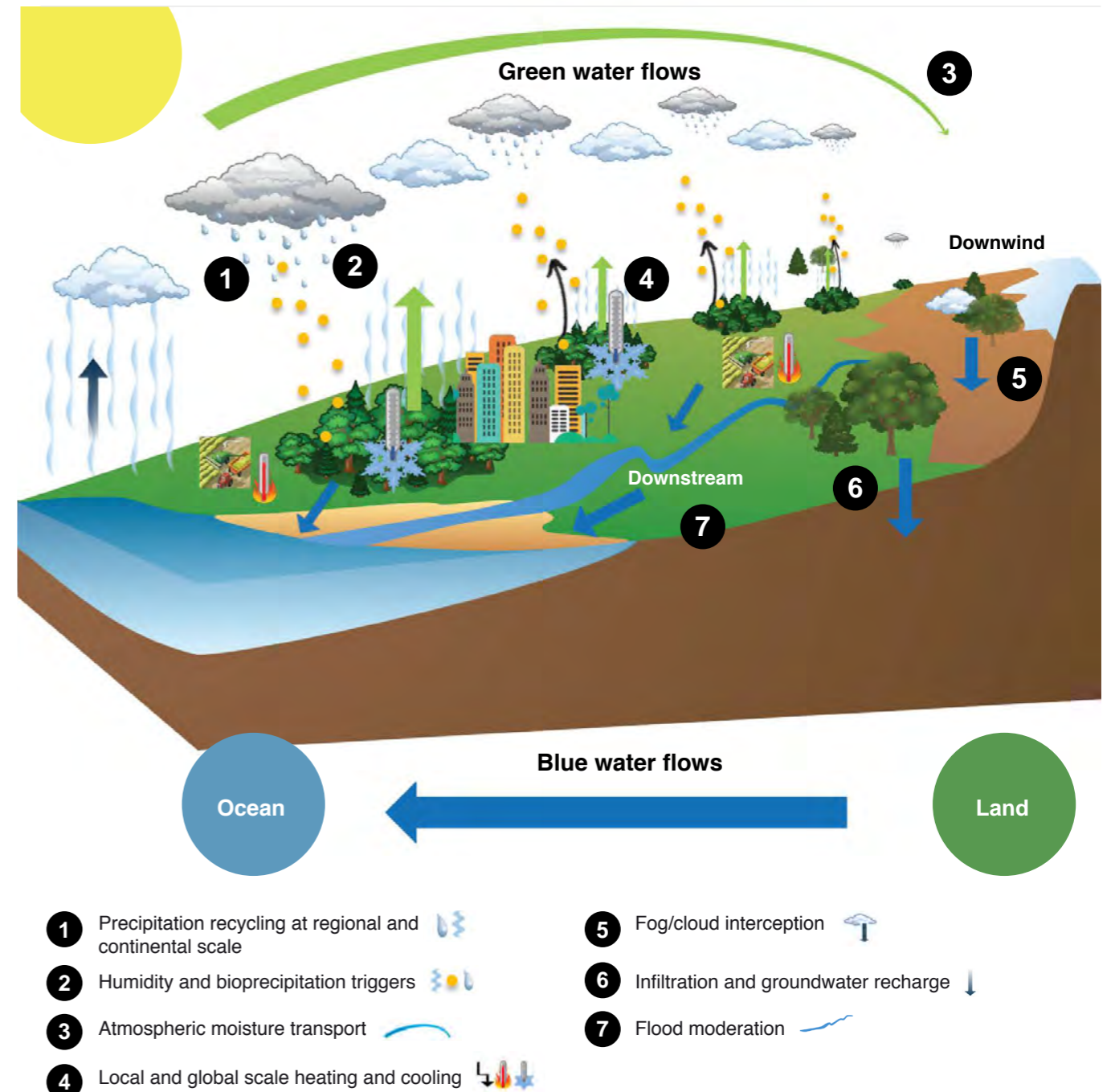
Figure 2. Forests balance blue and green water flows in the landscape. Green water: water that is intercepted or taken up by plants and returned to the atmosphere by evapotranspiration. Blue water: water that is running off or percolates and ends up in aquifers, rivers and lakes. Numbers 1-7 show the water cycle processes that are enhanced by trees and forests. (modified after Ellison et al. 2019 and Falkenmark & Rockström 2005) 2
